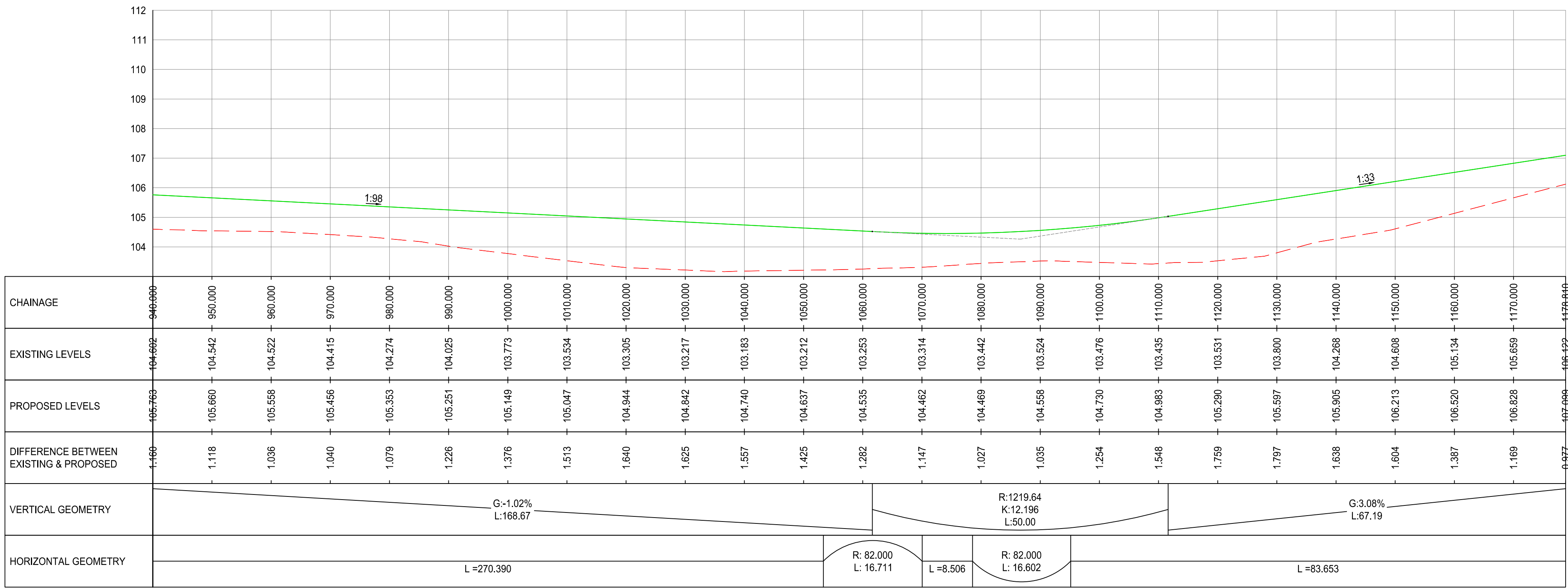
MAIN ROAD5 (CH 1000.0M - CH1078.0M) SCALE: H 1:500,V 1:100. DATUM: 103.000
